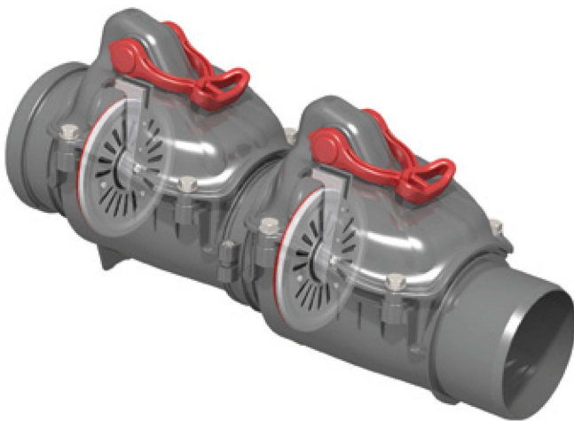
Double flap backwater \varnothing 110
