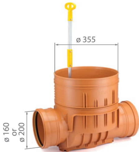
K35P16ZB dedicated for \varnothing 160 pipes
